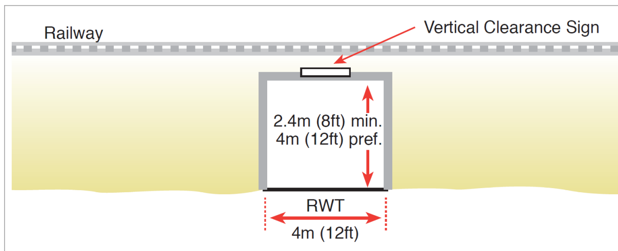
Figure 32: Rail-with-Trail Culvert under Tracks
